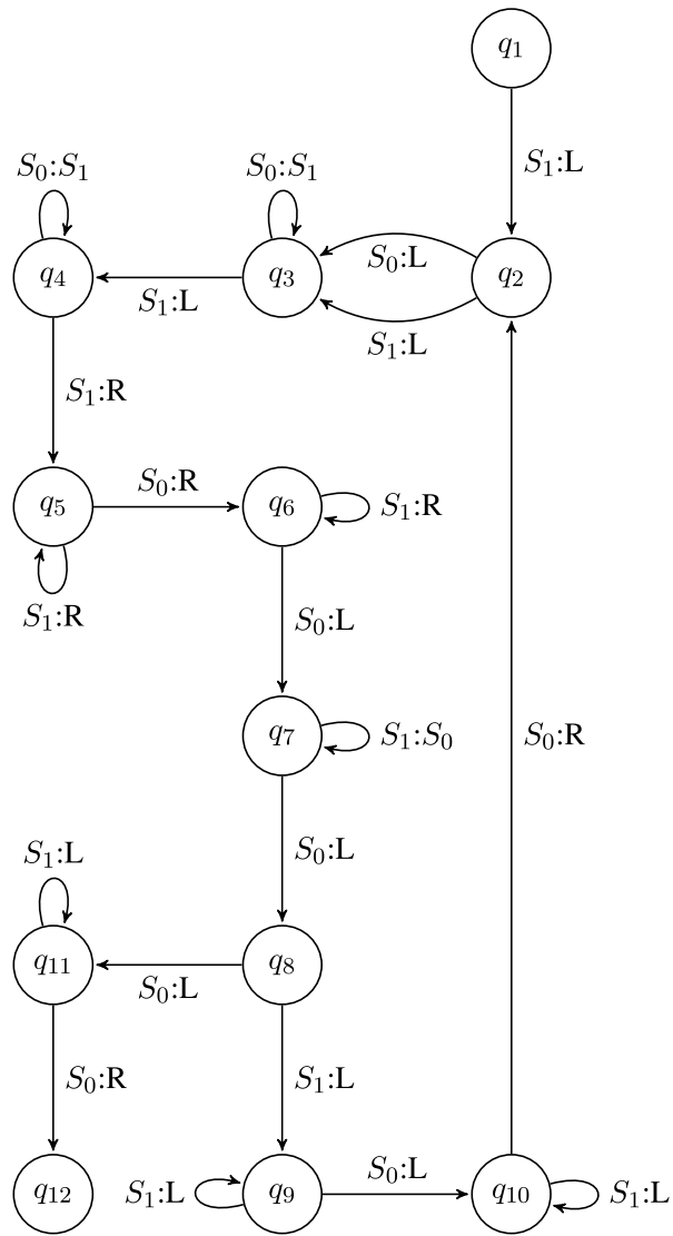
Figure 1: State Chart Diagram of Doubling
